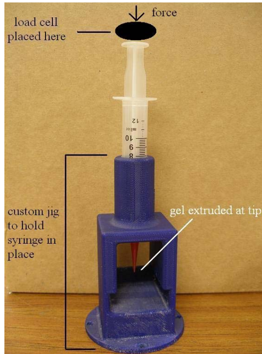
Fig. 2 Custom syringe-extrusion jig used in mechanical testing.
